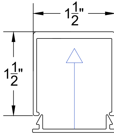
Bottom Channel
